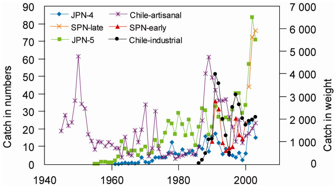
FIGURE 2. Catch by fishery in weight (t) and numbers of fish in the southeast swordfish SS2 model inputs.
