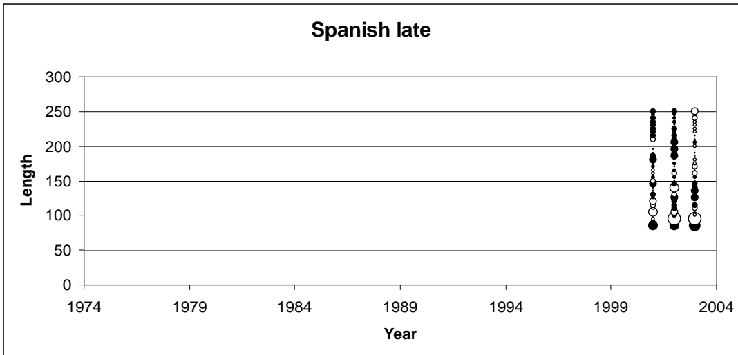
FIGURE 9.a.2. Residuals of the fit to the age and length-frequency data for Spanish fisheries scenario A.
