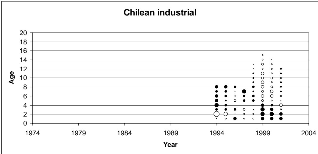
FIGURE 9.b.3. Residuals of the fit to the age and length-frequency data for Chilean fisheries in scenario B.
