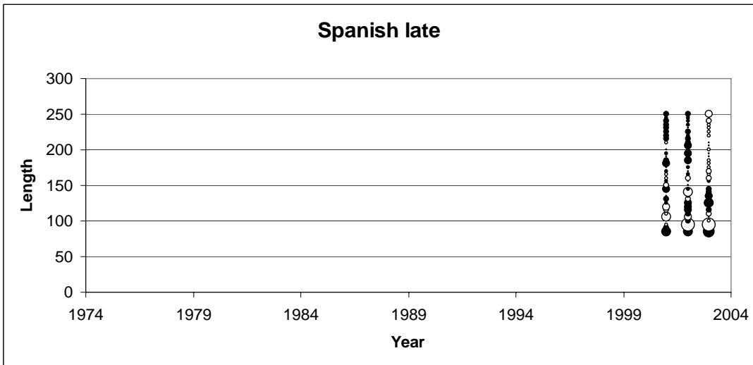
FIGURE 9.b.2. Residuals of the fit to the age and length-frequency data for Spanish fisheries in scenario B.
