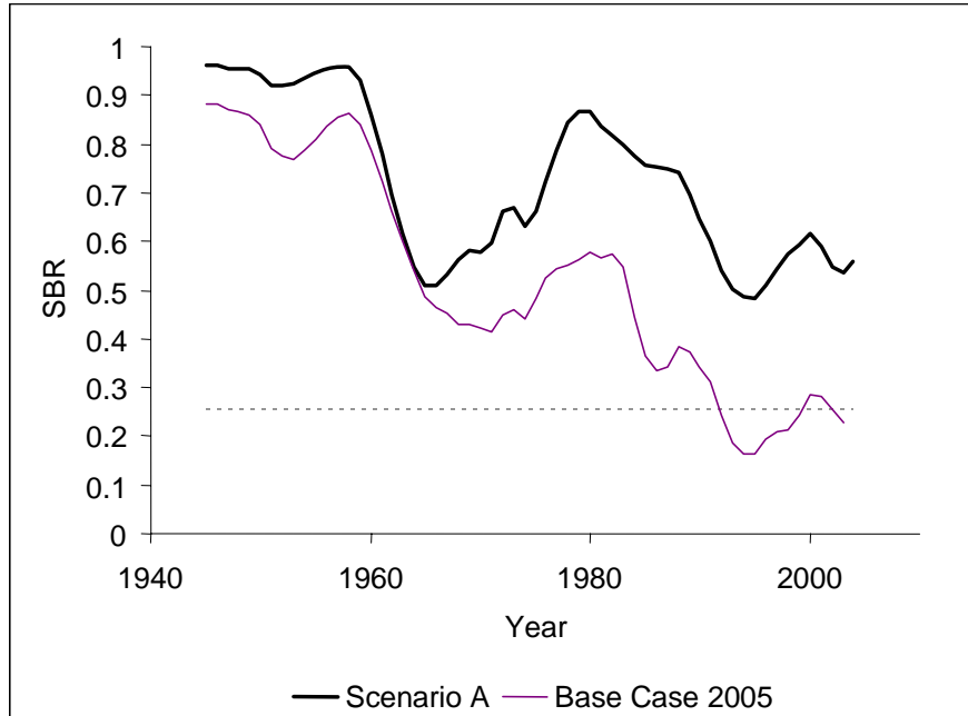
FIGURE 11. Comparison of trends in spawning biomass ratio (SBR) from SS2 model fits of current assessment scenario A to that of Hinton and Maunder (2005, Base case 2005).
