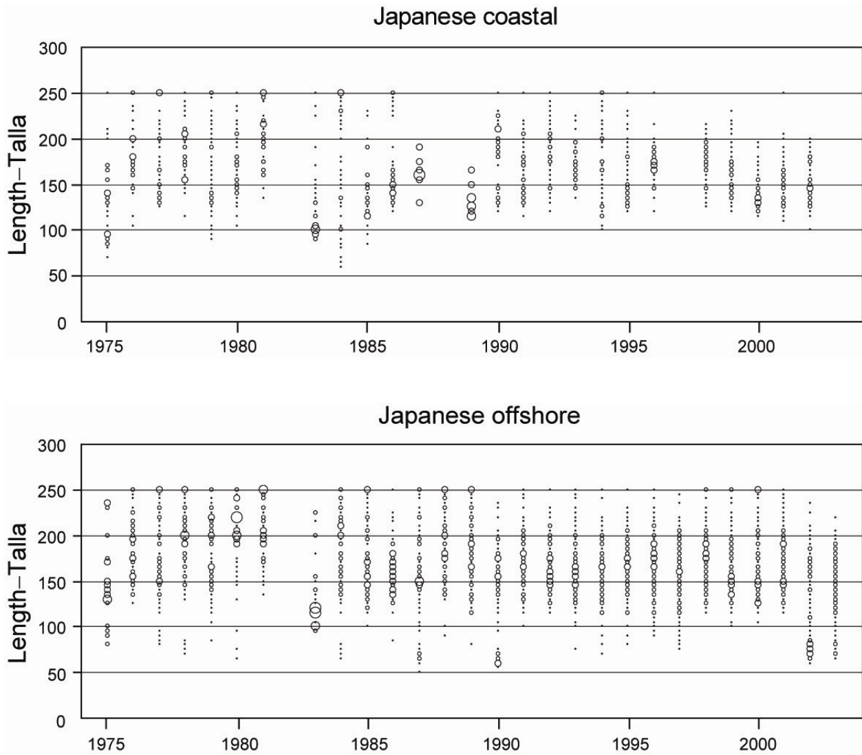
FIGURE 3.a. Length frequency (lower-jaw fork length) distributions of swordfish from the southern EPO from Japanese coastal and offshore fisheries
