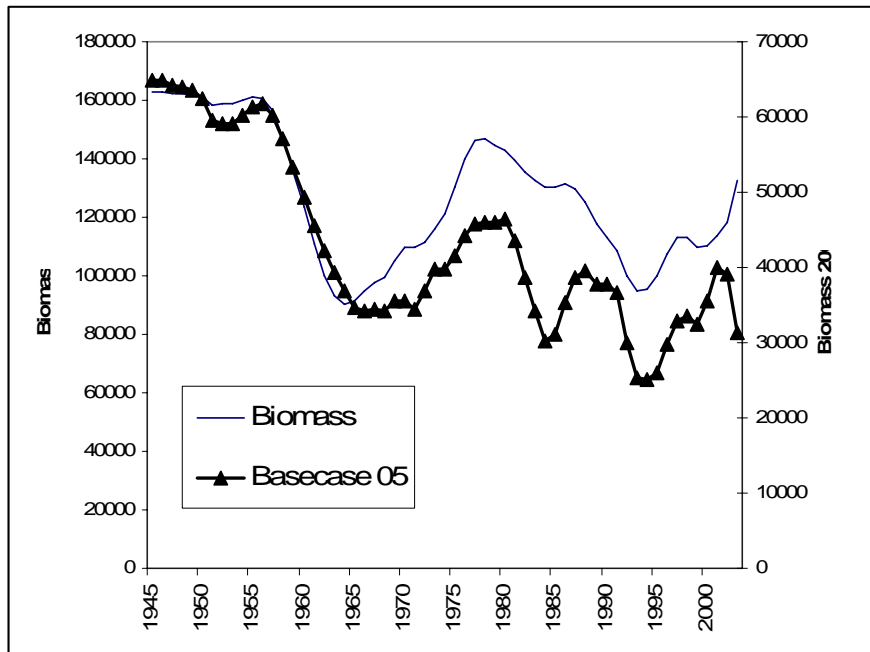
FIGURE 10. Comparison of trends in biomass in the current assessment to that of Hinton and Maunder (2005, Base case 05).
