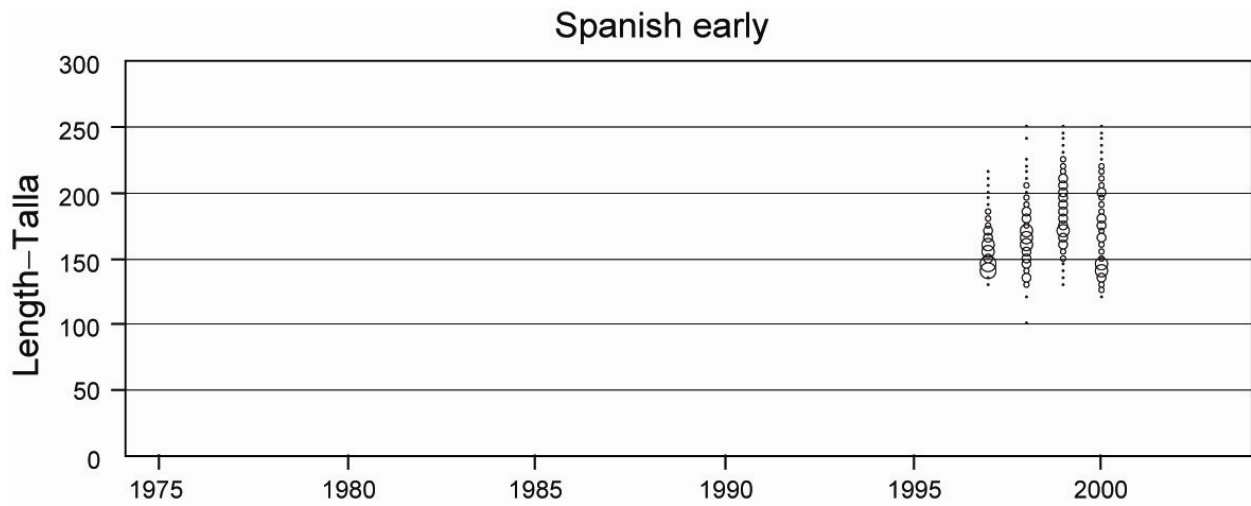
FIGURE 3.b. Length frequency (lower-jaw fork length) distributions of swordfish from the southern EPO from Spanish early and late period fisheries.
