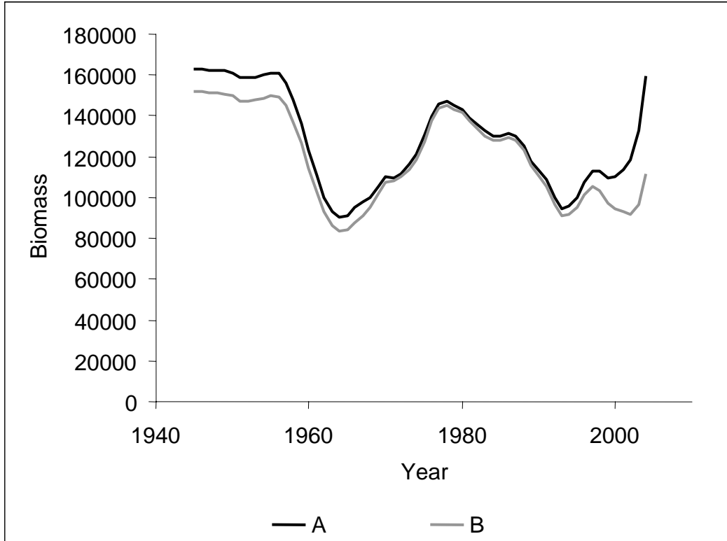
FIGURE 7. Estimated trend in vulnerable biomass (t) of swordfish in the southeast Pacific from SS2 model for two scenarios (A and B)
