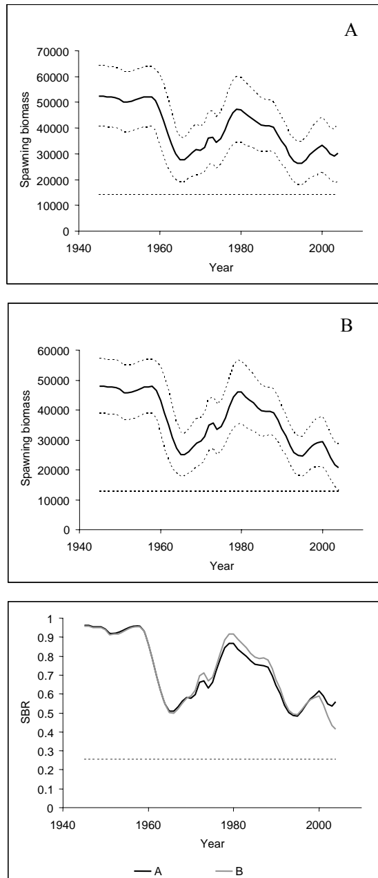
FIGURE 8. Trends in spawning biomass with 95% C.I. (scenarios A and B, upper panel) and spawning biomass ratio (SBR, lower panel) for swordfish in the south EPO.
