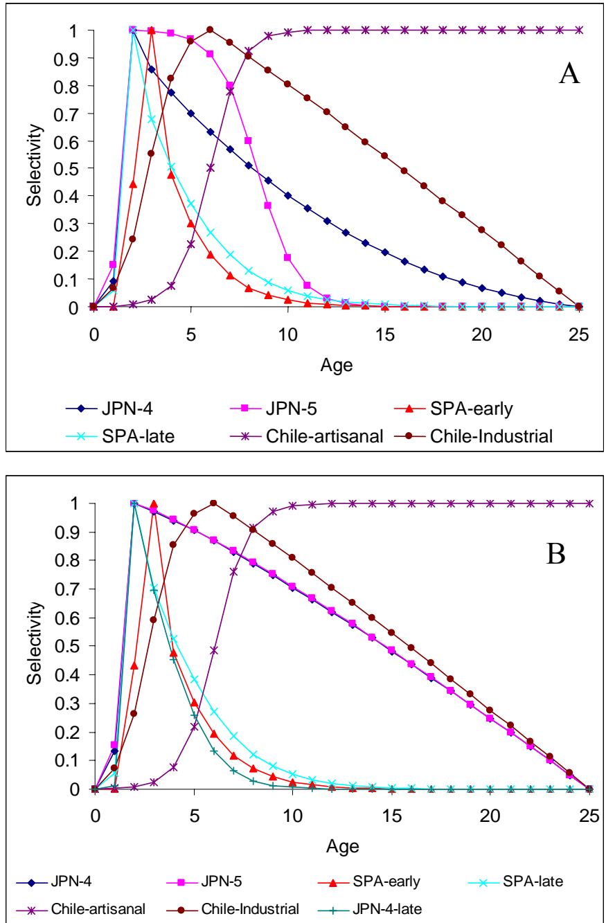
FIGURE 4. Selectivity for fisheries included in the SS2 model for swordfish in the southwest Pacific Ocean for scenarios A and B.
