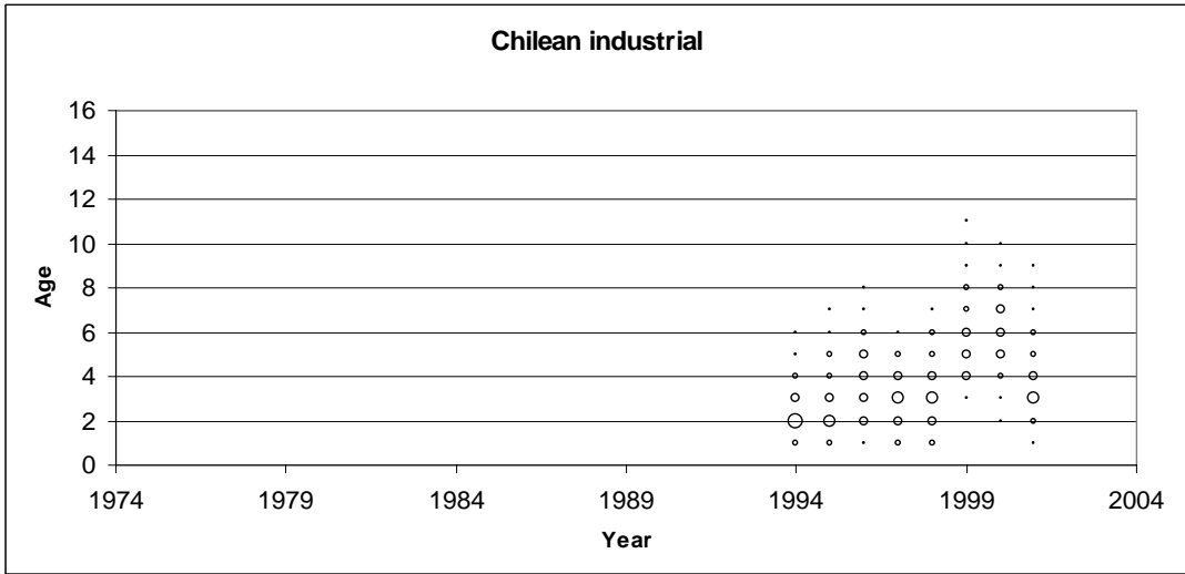
FIGURE 3.c. Age frequency distributions of swordfish from the southern EPO from Chilean artisanal and industrial longline fisheries.
