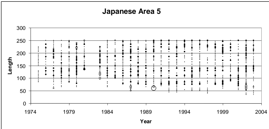
FIGURE 9.a.1. Residuals of the fit to the age and length-frequency data for Japanese fisheries scenario A.
