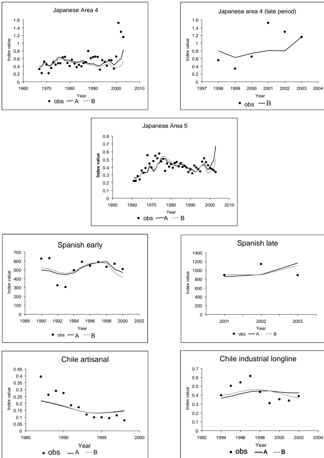
FIGURE 5. Observed catch rates and fitted indices for fisheries included in SS2 model of swordfish in the southeast Pacific Ocean for scenarios A and B.
