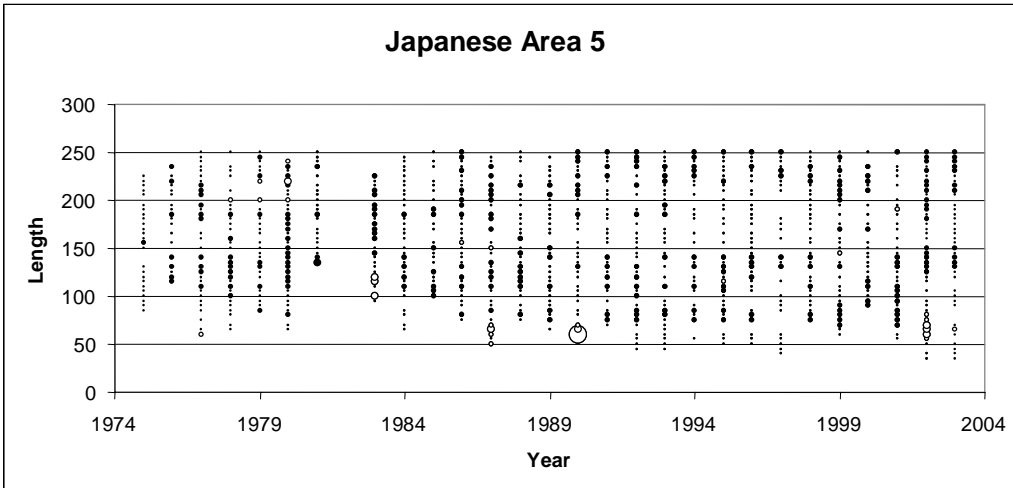
FIGURE 9.b.1. Residuals of the fit to the age and length-frequency data for Japanese fisheries in scenario B.
