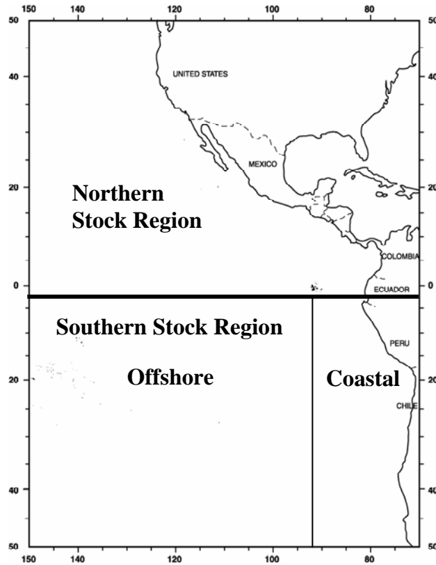
FIGURE 1. Subareas “Offshore” and “Coastal” of the EPO southern stock area (south of 5°S) in the SS2 model.
