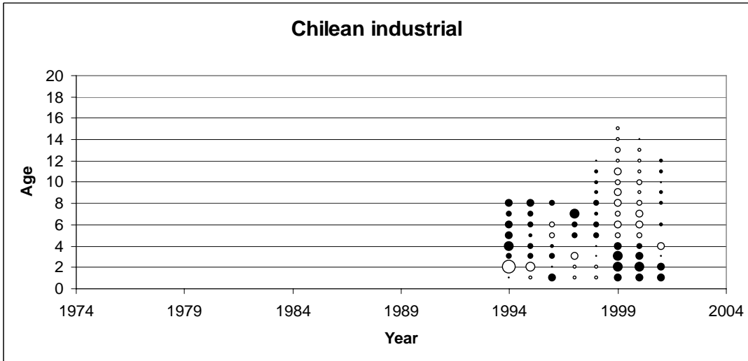
FIGURE 9.a.3. Residuals of the fit to the age and length-frequency data for Chilean fisheries scenario A.
