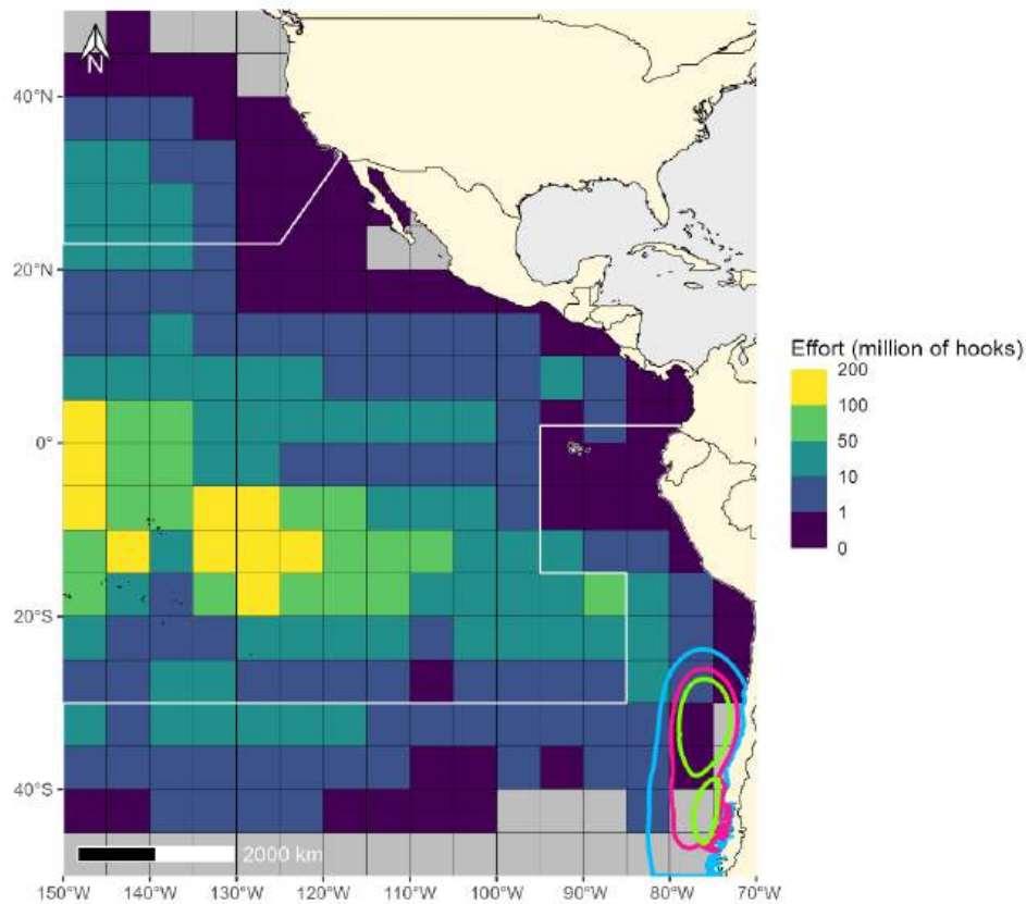
Annex 2 Figure 4. Overlapping 95% (blue line), 75% (pink line), and 50% (light green line) isopleths of adult non-breeding Black-browed Albatross ( Thalassarche melanophris ) based on GLS tracks with longline fishing effort data (in number of hooks) from logbooks reported in 5°x5° grid cells by CPCs from 2000-2023. The areas north of the northern white line and south of the southern white line represent where two mitigation measures are required under C-11-02.
