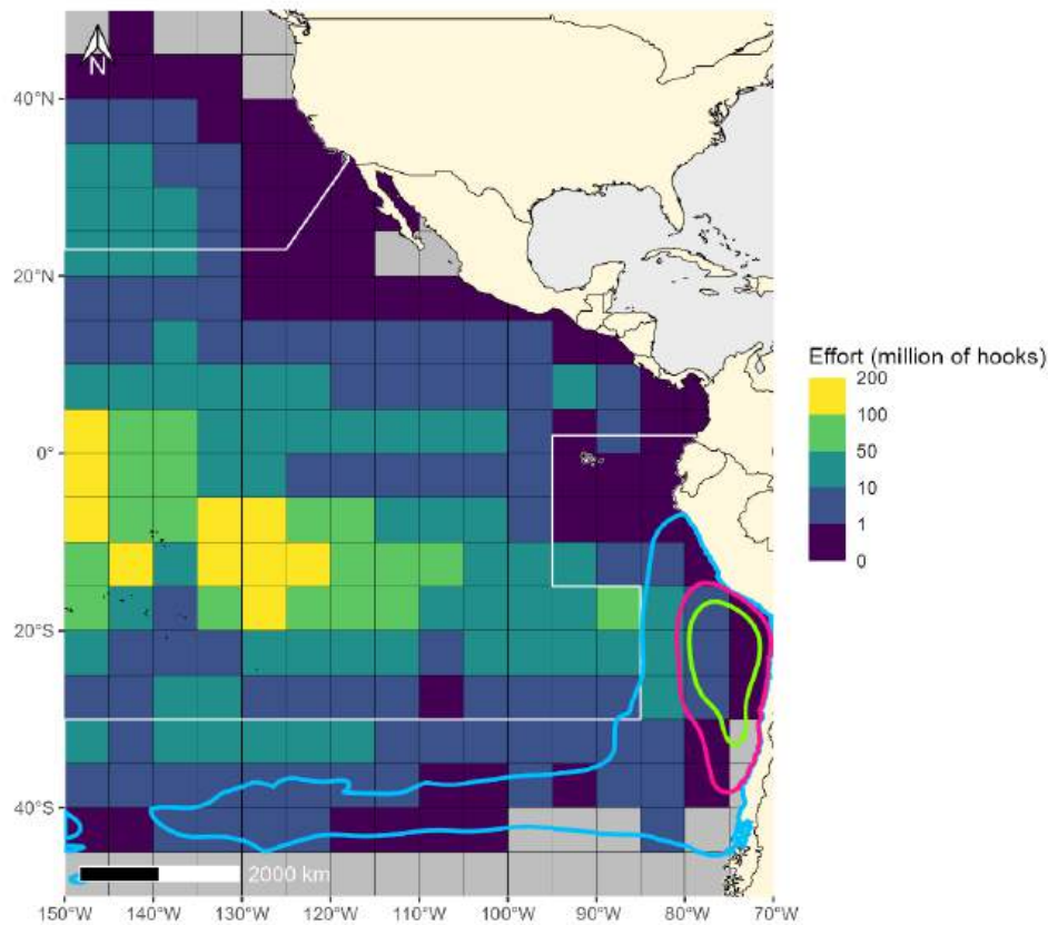
Annex 2 Figure 6. Overlapping 95% (blue line), 75% (pink line), and 50% (light green line) isopleths of adult non-breeding Buller's Albatross ( Thalassarche bulleri ) based on GLS tracks with longline fishing effort data (in number of hooks) from logbooks reported in 5°x5° grid cells by CPCs from 2000-2023. The areas north of the northern white line and south of the southern white line represent where two mitigation measures are required under C-11-02.
