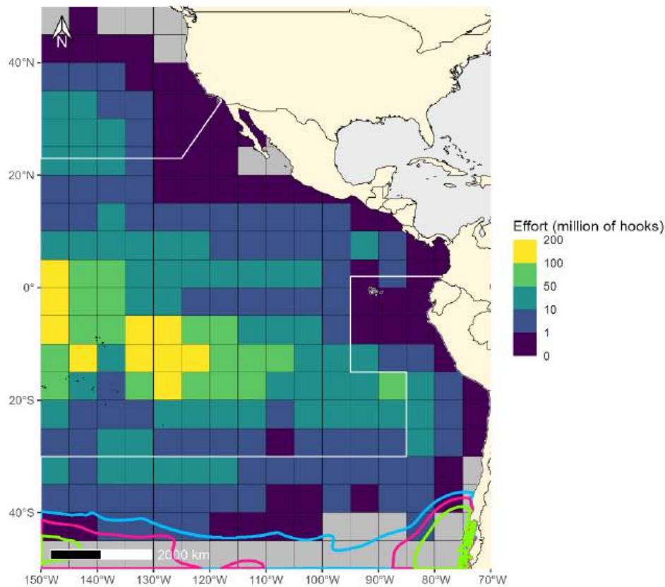
Annex 2 Figure 14. Overlapping 95% (blue line), 75% (pink line), and 50% (light green line) isopleths of adult non-breeding Wandering Albatross ( Diomedea exulans ) based on GLS tracks with longline fishing effort data (in number of hooks) from logbooks reported in 5°x5° grid cells by CPCs from 2000-2023. The areas north of the northern white line and south of the southern white line represent where two mitigation measures are required under C-11-02.
