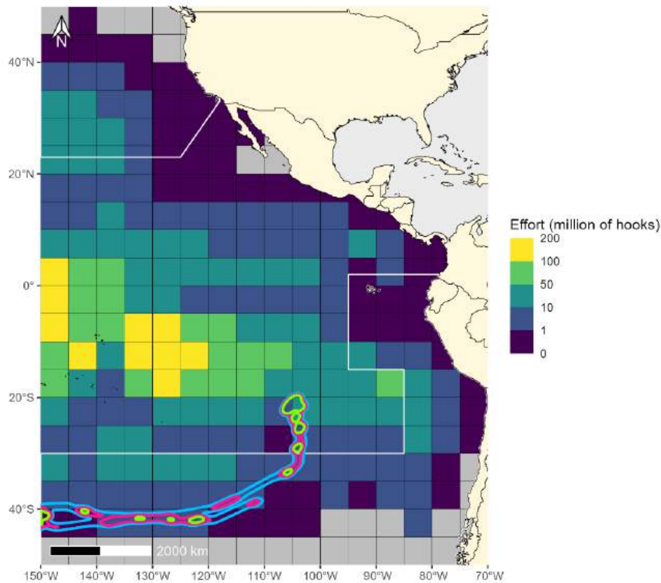
Annex 2 Figure 7. Overlapping 95% (blue line), 75% (pink line), and 50% (light green line) isopleths of adult non-breeding Buller's Albatross ( Thalassarche bulleri ) based on GPS/PTT tracks with longline fishing effort data (in number of hooks) from logbooks reported in 5°x5° grid cells by CPCs from 2000-2023. The areas north of the northern white line and south of the southern white line represent where two mitigation measures are required under C-11-02.
