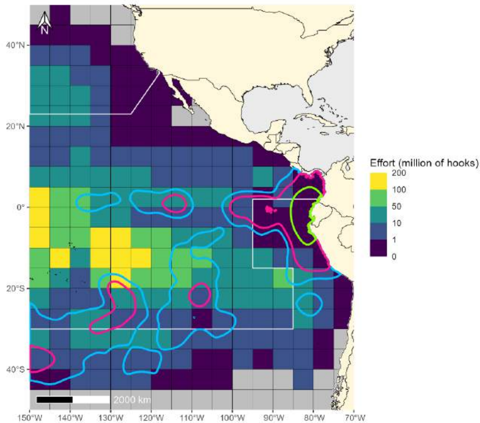
Annex 2 Figure 5. Overlapping 95% (blue line), 75% (pink line), and 50% (light green line) isopleths of adult non-breeding Black Petrel ( Procellaria parkinsoni ) based on GLS tracks with longline fishing effort data (in number of hooks) from logbooks reported in 5°x5° grid cells by CPCs from 2000-2023. The areas north of the northern white line and south of the southern white line represent where two mitigation measures are required under C-11-02.
