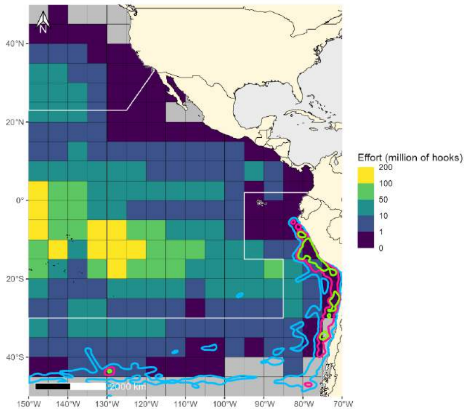
Annex 2 Figure 9. Overlapping 95% (blue line), 75% (pink line), and 50% (light green line) isopleths of adult non-breeding Chatham Albatross ( Thalassarche eremita ) based on GPS/PTT tracks with longline fishing effort data (in number of hooks) from logbooks reported in 5°x5° grid cells by CPCs from 2000-2023. The areas north of the northern white line and south of the southern white line represent where two mitigation measures are required under C-11-02.
