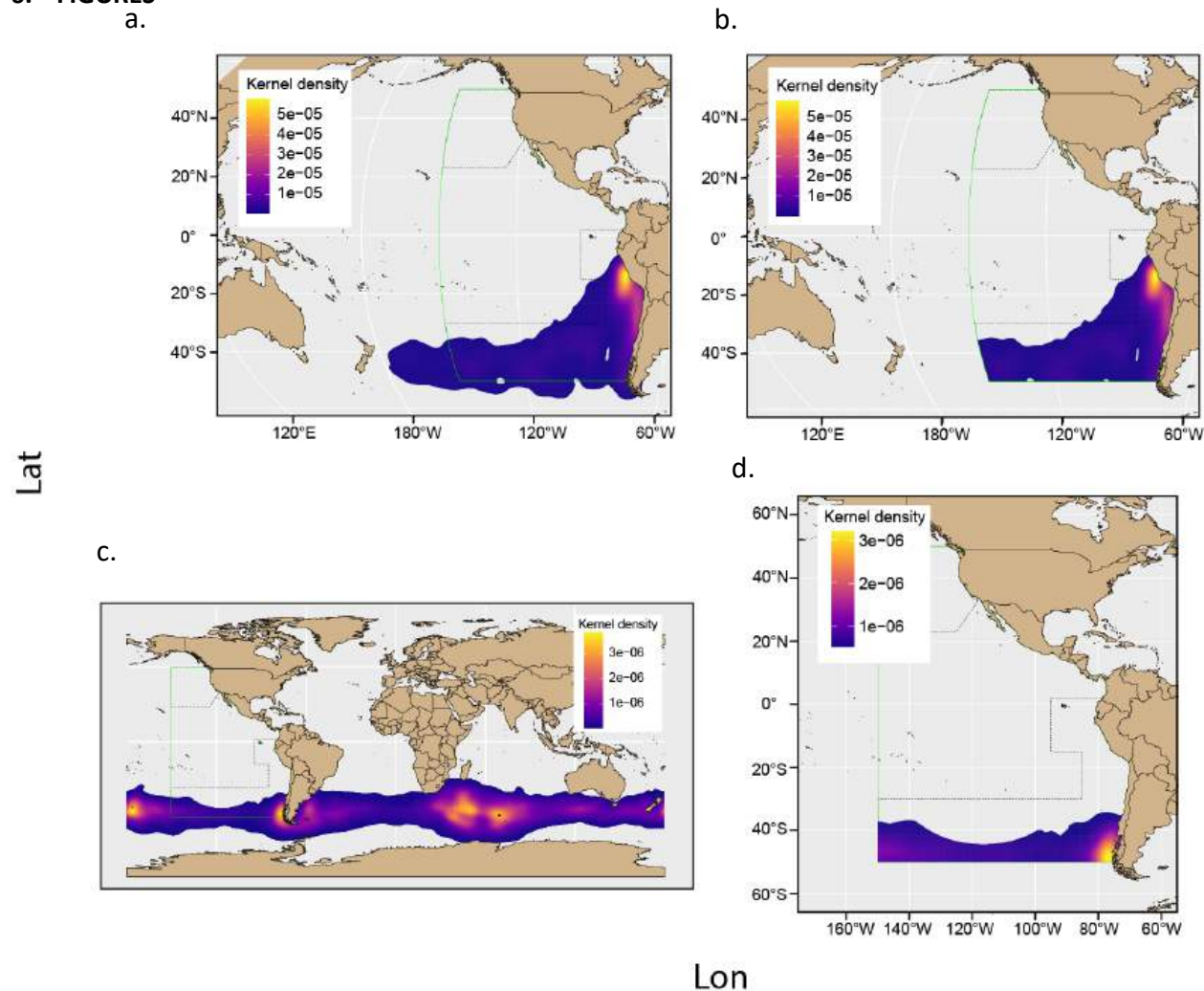
FIGURE 1. Two representative global (a,c) and cropped (b,d) utilization distributions (UDs) for the adult non-breeding Chatham Albatross, Thalassarche eremita , (a,b) and Wandering Albatross, Diomedea exulans , (c,d). The density scales will likely differ between the global and cropped UD because the range of density values likely changes after cropping to the IATTC area. Green line outlines the IATTC Convention Area, while the areas north of the northern black dashed line and south of the southern black dashed line represent where two mitigation measures are required under C-11-02.
