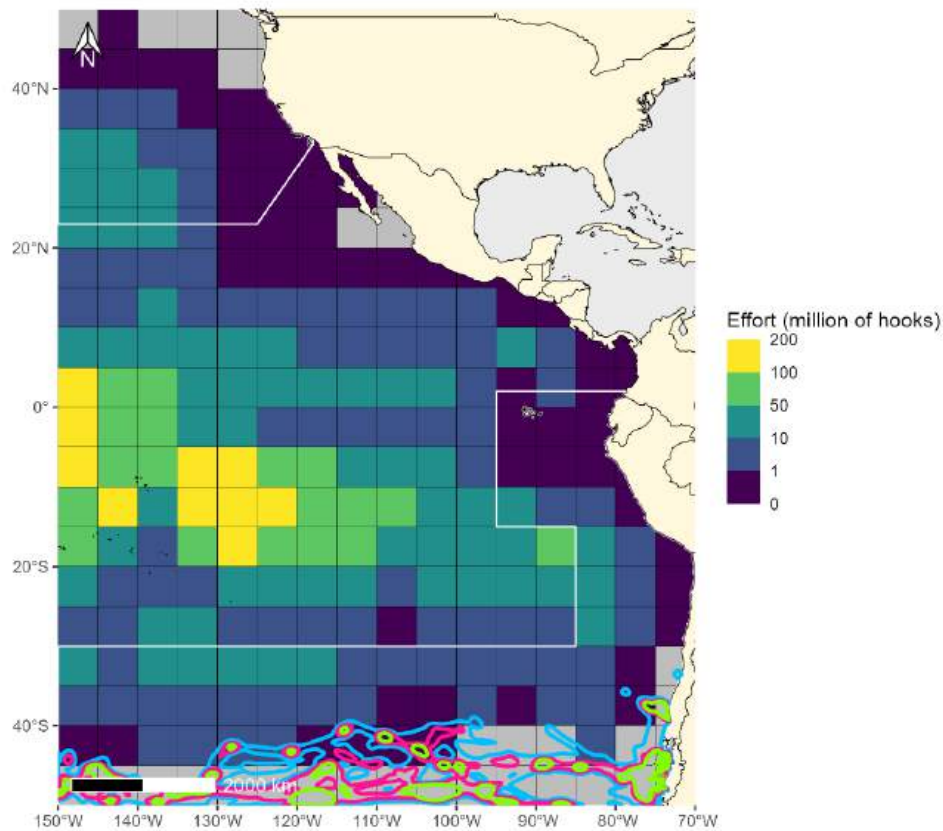
Annex 2 Figure 11. Overlapping 95% (blue line), 75% (pink line), and 50% (light green line) isopleths of juvenile Northern Giant Petrel ( Macronectes halli ) based on GLS tracks with longline fishing effort data (in number of hooks) from logbooks reported in 5°x5° grid cells by CPCs from 2000-2023. The areas north of the northern white line and south of the southern white line represent where two mitigation measures are required under C-11-02.
