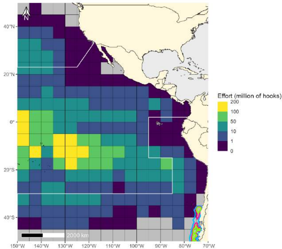
Annex 2 Figure 3. Overlapping 95% (blue line), 75% (pink line), and 50% (light green line) isopleths of adult breeding Black-browed Albatross ( Thalassarche melanophris ) based on GPS/PTT tracks with longline fishing effort data (in number of hooks) from logbooks reported in 5°x5° grid cells by CPCs from 2000-2023. The areas north of the northern white line and south of the southern white line represent where two mitigation measures are required under C-11-02.
