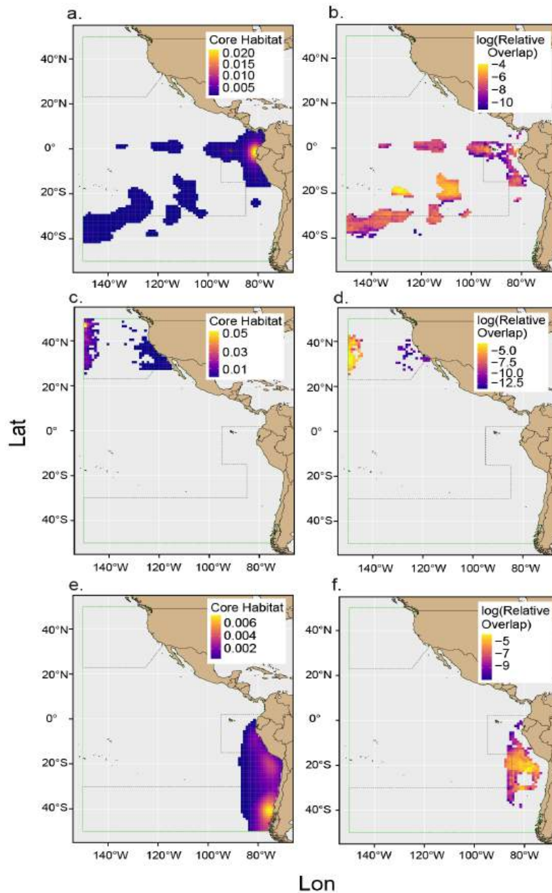
FIGURE 4. Core habitat (a, c, e) extracted from utilization distributions and associated relative overlap (b, d, f) with Global Fishing Watch estimated longline fishing effort for adult non-breeding Black Petrel, Procellaria parkinsoni , (a, b), breeding Laysan Albatross, Phoebastria immutabilis , (c, d), and adult non-breeding White-chinned Petrel, Procellaria aequinoctialis , (e, f). The highest relative overlap are areas in yellow. The areas north of the northern black dashed line and south of the southern black dashed line represent where two mitigation measures are required under C-11-02 .
