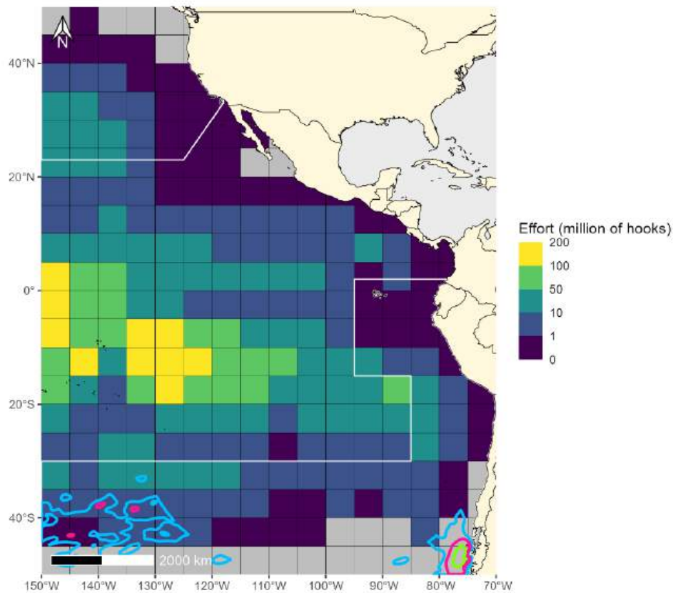
Annex 2 Figure 13. Overlapping 95% (blue line), 75% (pink line), and 50% (light green line) isopleths of juvenile Wandering Albatross ( Diomedea exulans ) based on GPS/PTT tracks with longline fishing effort data (in number of hooks) from logbooks reported in 5°x5° grid cells by CPCs from 2000-2023. The areas north of the northern white line and south of the southern white line represent where two mitigation measures are required under C-11-02.
