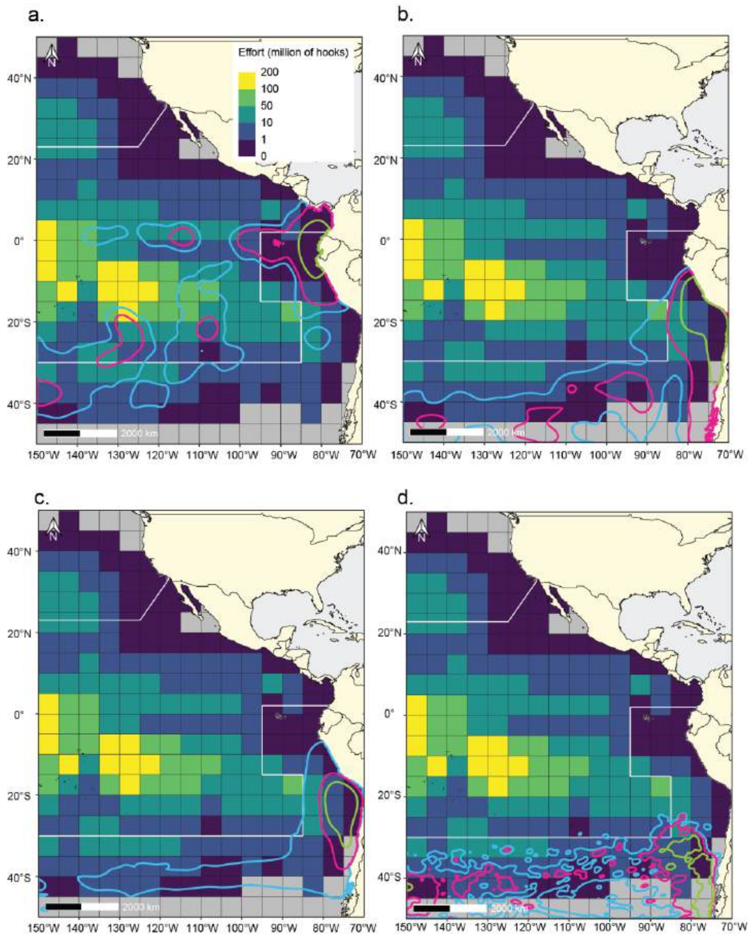
FIGURE 3. Overlapping 95% (blue line), 75% (pink line), and 50% (light green line) isopleths of a) adult non-breeding Black Petrel, Procellaria parkinsoni , b) Chatham Albatross, Thalassarche eremita , c) Buller's Albatross, Thalassarche bulleri , and d) Antipodean Albatross, Diomedea antipodensis , with longline fishing effort data (in number of hooks) from logbooks reported in 5°x5° grid cells by CPCs from 2000–2023. The areas north of the northern white line and south of the southern white line represent where two mitigation measures are required under C-11-02 .
