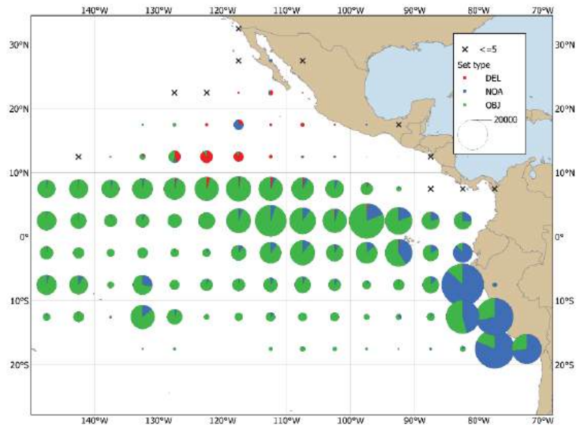
FIGURE A-2b. Annual distributions of the purse-seine catches of skipjack, by set type, 2024. The sizes of the circles are proportional to the amounts of skipjack caught in those 5° by 5° areas.
