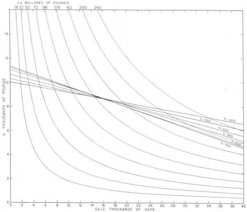
Figure 4. Lines of equilibrium conditions calculated for different assumed values of annual rate of fishing mortality (at 25,000 standard days' fishing). Lines for f = 0.614 and f = 0.800 not shown (see Table 5); both fall between lines for f = 0.600 and f = 0.700 .
