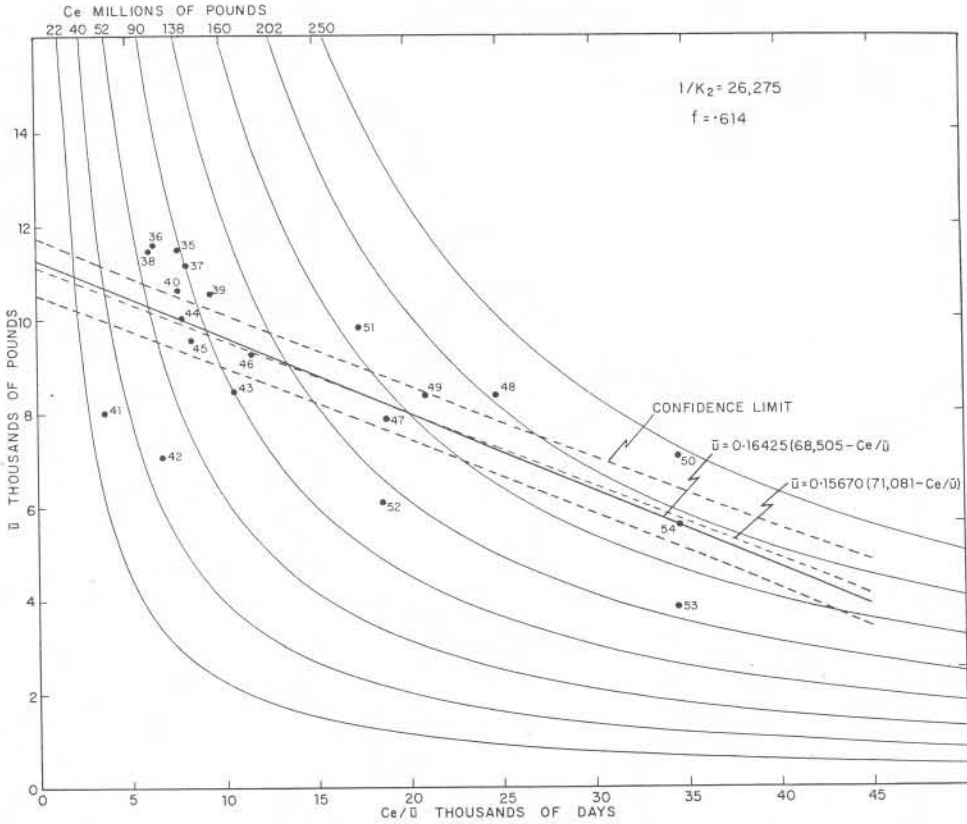
Figure 3. Relationships among fishing intensity, abundance, and equilibrium catch, assuming 1/k_2 = 26,275 . Points indicate values computed for each year 1935-1954. Solid line is estimated functional relationship between fishing intensity and average abundance under equilibrium conditions. Broken lines indicate the values of average abundance estimated for given values of fishing intensity, with the 90% confidence limits on the estimates.
