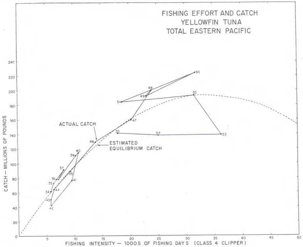
Figure 2. Relationship between fishing intensity and total catch. Points connected by solid line indicate actual values for each year 1934-1955. Broken line is estimated functional relationship between fishing intensity and average equilibrium catch.
