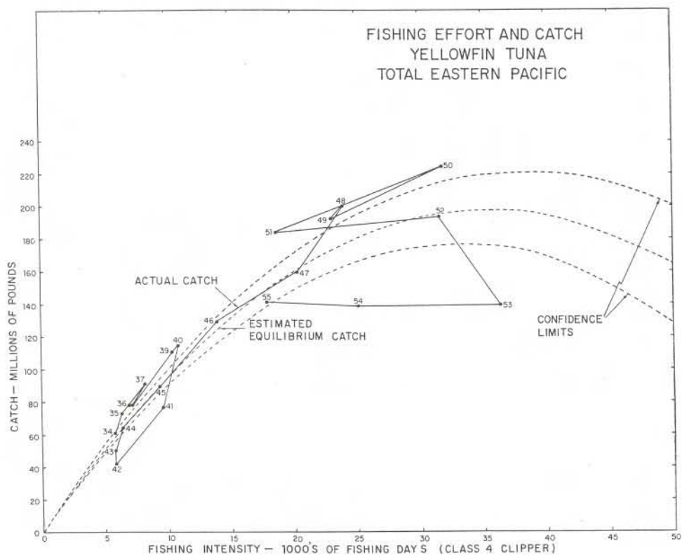
Figure 5. Average equilibrium catch predicted for given values of fishing intensity, with 90% confidence limits (broken lines), together with actual values of effort and catch for the years 1934-1955 (points connected by solid line).
