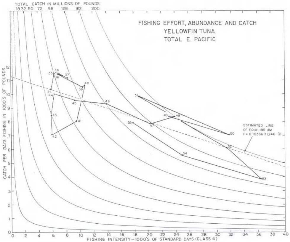
Figure 1. Relationships among fishing intensity, abundance and total catch. Points connected by solid line indicate actual values for each year 1934-1955. Broken line is estimated functional relationship between fishing intensity and average abundance under equilibrium conditions.
