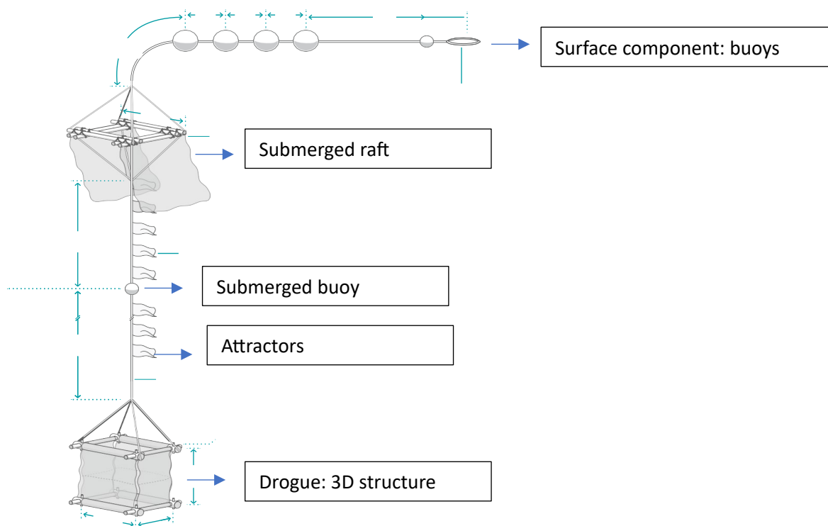
Figure 1. Scheme of the bio-FAD tested, called jelly-FAD.
