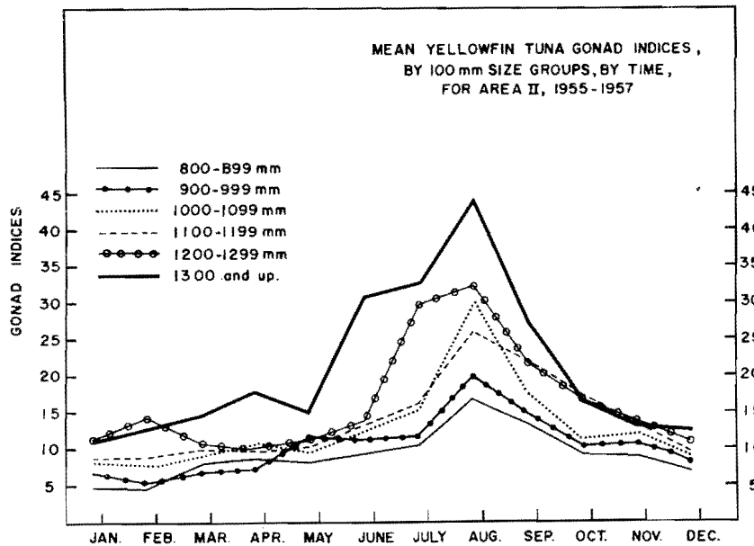
FIGURE 14. Mean gonad indices for yellowfin tuna, by size groups, for Area 02, (Revilla Gigedo Islands).
