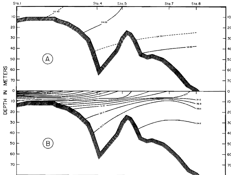
FIGURE 16. Typical salinity profiles for the Gulf of Nicoya during (A) the dry season, and (B) the rainy season.
