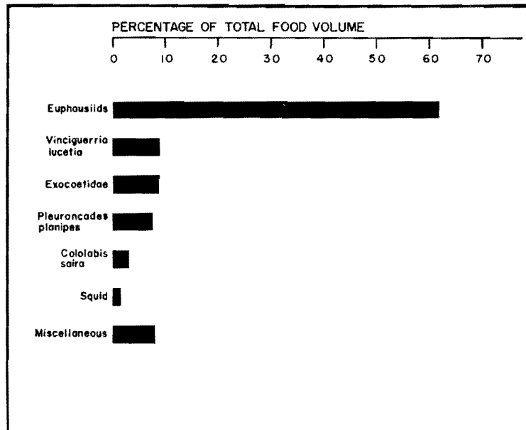
FIGURE 13. Relative importance, by volume, of the major components of skipjack food.
