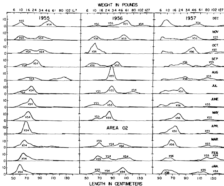
FIGURE 8. Size composition of yellowfin tuna landed from Area 02 (Revilla Gigedo Islands) during 1955-1957, indicating the growth of age-classes, and the occurrence of two age-classes in some years.
