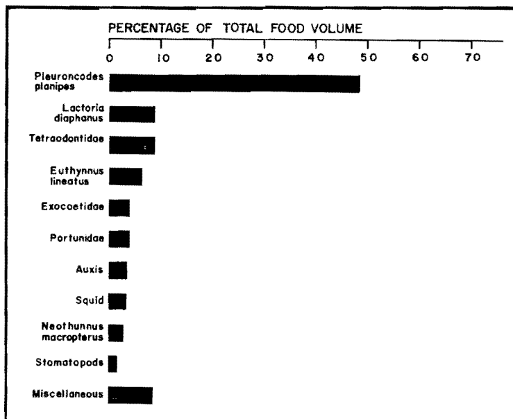
FIGURE 12. Relative importance, by volume, of the major components of yellowfin tuna food.
