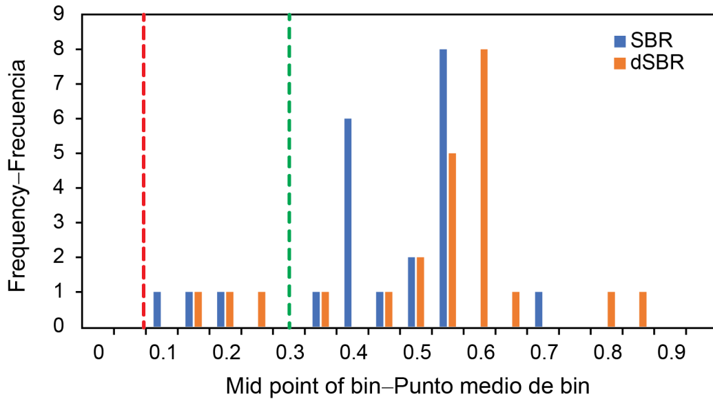
FIGURE 36. Frequency distribution of the estimates of SBR and dSBR. The vertical lines are the limit reference point (0.077) and the proxy target reference point (0.30).
