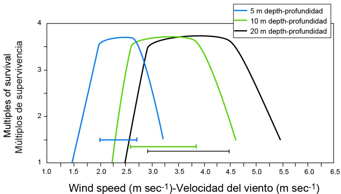
FIGURE 5. Relationship between microturbulence (estimated in the top panel as the turbulent dissipation rate and converted in the bottom panel to wind speed) and survival of yellowfin larvae during the first week of feeding. The survival curve is a smoothed, composite curve representing the mean survival estimated during 4 trials over 3 years.
