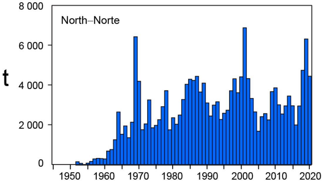
FIGURE G-2. Retained catches of swordfish in the North EPO for 1945–2020.
