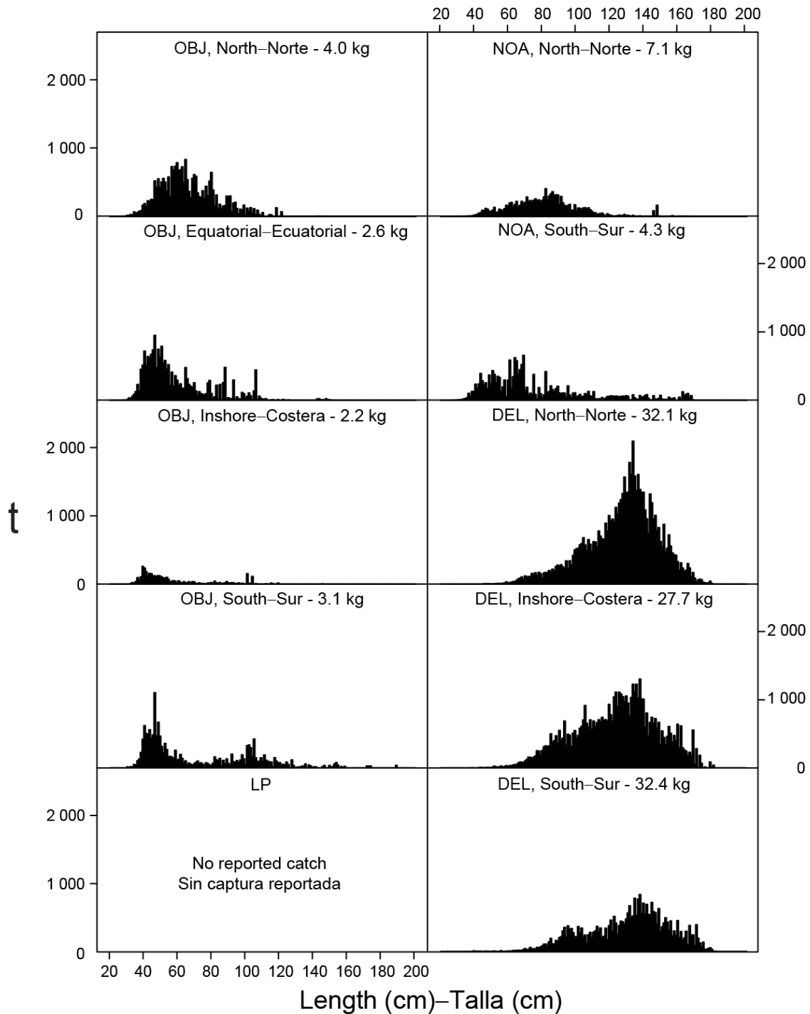
FIGURE A-6a. Estimated size compositions of the yellowfin caught in the EPO during 2021 for each fishery designated in Figure A-5. The value at the top of each panel is the average weight of the fish in the samples.
