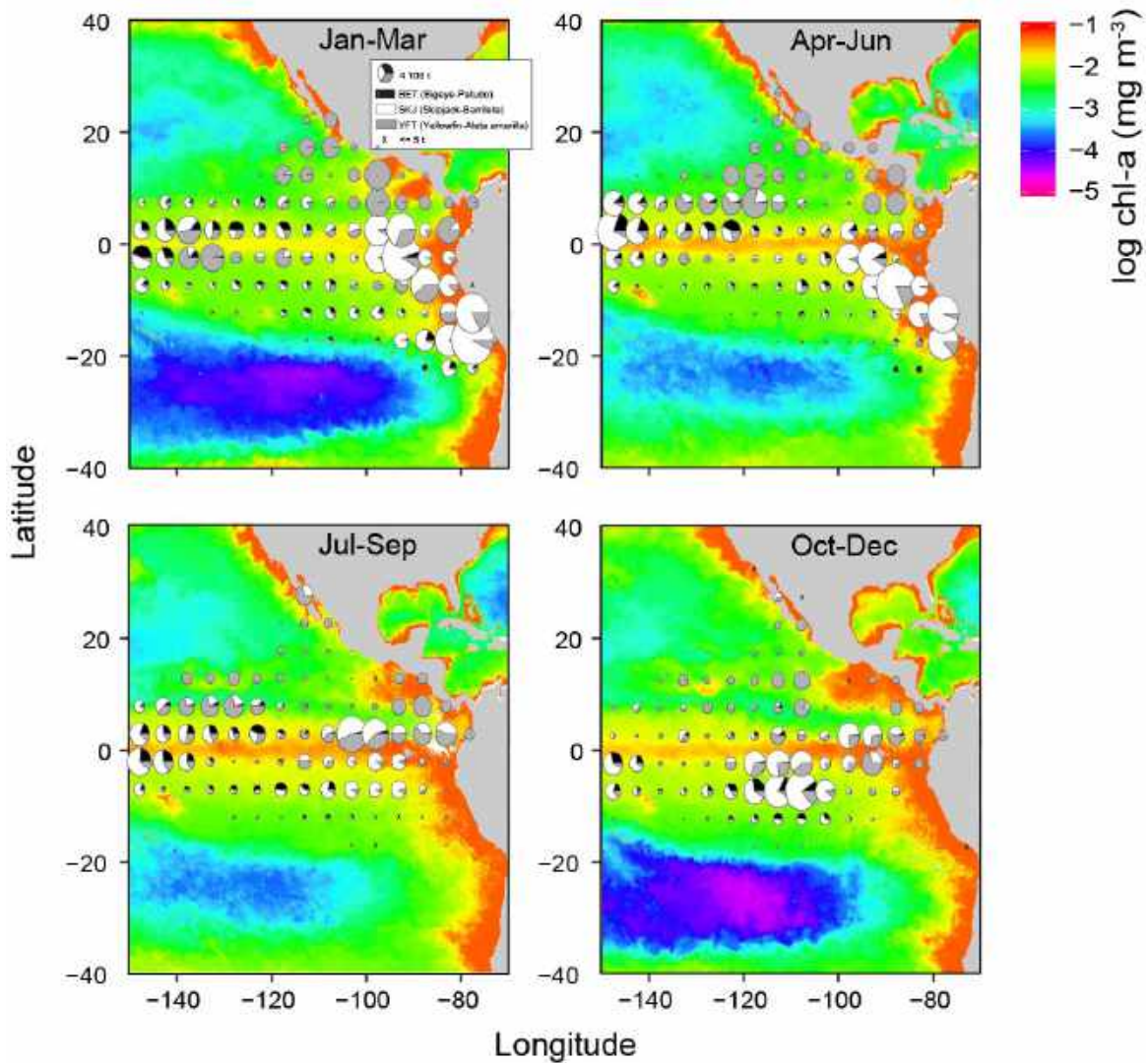
FIGURE L-11. Mean log chlorophyll-a concentration (in \text{mg m}^{-3} ) for each quarter during 2020 with catches of tropical tunas overlaid. Chlorophyll data obtained from NOAA CoastWatch on January 25, 2021, “Chlorophyll, NOAA, VIIRS, Science Quality, Global, Level 3, 2012-present, Monthly”, NOAA NMFS SWFSC ERD, https://coastwatch.pfeg.noaa.gov/erddap/info/nedisVHNSQchlaMonthly/index.html .
