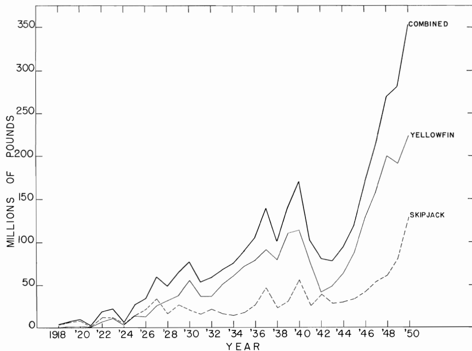
FIGURE 1—Catch of yellowfin and skipjack tuna from the Eastern Pacific Ocean, 1918 to 1950.
