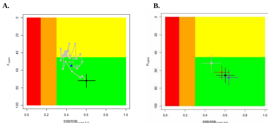
Figure F-3. (A) Stock status phase plot showing the status of the north Pacific albacore ( Thunnus alalunga ) stock relative to the biomass-based threshold ( 30\%SSB_{current, F=0} ) and limit ( 14\%SSB_{current, F=0} ) reference points, and fishing intensity-based target reference point ( F_{45\%SPR} ) over the modeling period (1994 – 2024). Blue triangle indicates the start year (1994) and black circle with 95% confidence intervals indicates the terminal year (2024). (B) Stock status plot showing current stock status and 95% confidence intervals of the base case model (black circle), a sensitivity run an important sensitivity run of CV = 0.06 for L_{inf} in the growth model (gray), an important sensitivity run with two initial fishing mortality parameters (red), and a model representing an update of the 2023 base case model to 2026 data (purple). Red zones in both panels indicate female SSBs falling below the limit reference point while the orange zones indicate female SSBs between the threshold and limit reference points. Green zones indicate female SSBs above the threshold reference point and fishing intensity levels below the target reference point. Yellow areas indicate female SSBs above the threshold reference point and fishing intensity levels above the target reference point. The Fs in this figure are indicators of fishing intensity based on spawning potential ratio (SPR) and calculated as %SPR. SPR is the ratio of the equilibrium SSB per recruit that would result from the estimated F-at-age relative to that of an unfished population. A higher %SPR indicates lower fishing intensity. Current fishing intensity values and SSB/SSB_{current, F=0} ratios in (B) were calculated as the average during 2021–2023 ( F_{\%SPR, 2021-2023} ) and 2024 ( SSB_{2024}/SSB_{current, F=0} ), respectively. The model representing an update of the 2023 base case model is similar to but not identical to the 2023 base case model due to changes in data preparation and model structure.
