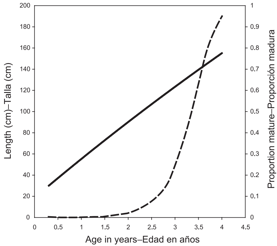
FIGURE 1. Relationships between length and estimated age of bigeye (solid curve) and proportion of female bigeye tuna mature and estimated age (dashed curve).
