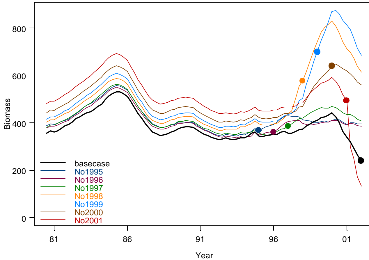
Figure 11: Estimated biomass trajectories from the retrospective analyses. The solid points represent the last estimate for which data were available. Lines after the point represent predictions based on observed effort.
