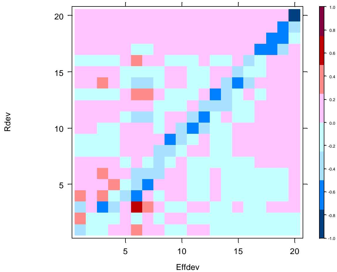
Figure 8: Correlations between estimates of recruitment deviates and effort deviates for the discard fishery from the basecase model for bigeye for the last twenty quarters. The top right corner represents the most recent period.
