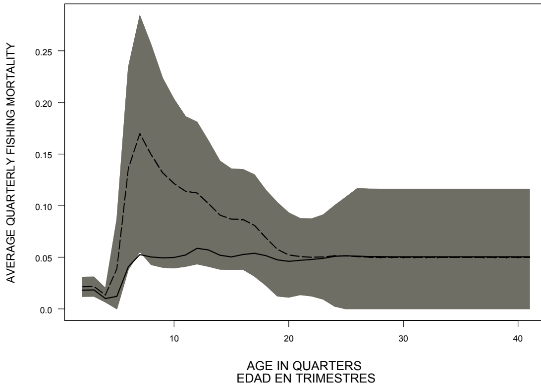
FIGURE C.1. Average quarterly age-specific fishing mortality used in the yield calculations and projections for the basecase (solid line) and sensitivity analysis (dashed line). The basecase is based on average catchability over the whole modeling time period and the sensitivity is based on average catchability over the last two years. The shaded area represents the 95% confidence intervals for the estimated average quarterly age-specific fishing mortality used in the sensitivity analysis.
