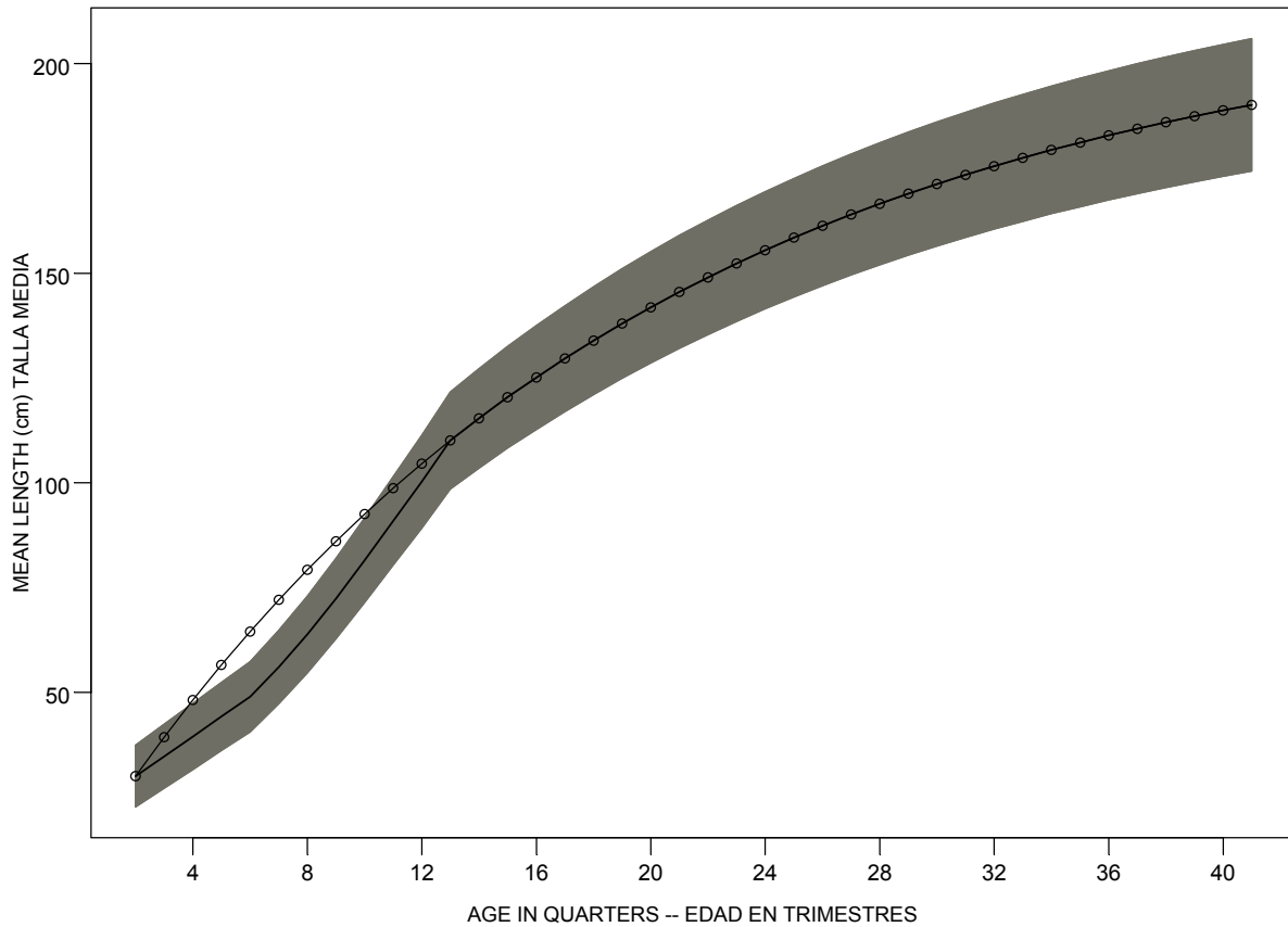
FIGURE 4.13. Estimated average lengths at age for bigeye tuna in the EPO. The filled area indicates the range of lengths estimated to be covered by two standard deviations of the length at age. The line with circles represent the growth curve from Suda and Kume (1967), which is used as a prior.
