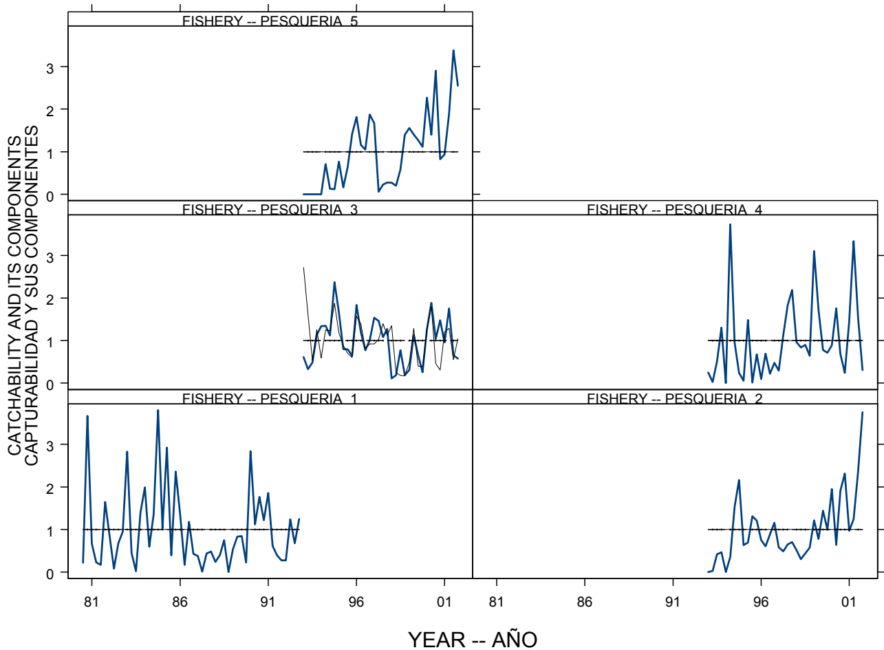
FIGURE 4.7a. Trends in catchability ( q ) for the 13 fisheries that take bigeye tuna in the EPO. The estimates are scaled to the first estimate of q for each fishery (dashed line). The thin line (Fishery 3 only) illustrates the environment index for q . The bold lines include random effects, and illustrate the overall trends in catchability. When the thin lines and bold lines follow the same trend the environmental conditions may be considered to explain patterns in catchability.
