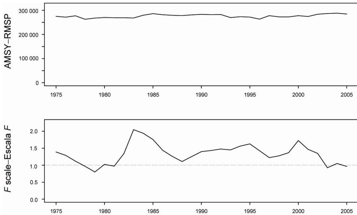
FIGURE B-7. AMSY (upper panel), 1975-2005, and the change (increase or reduction) in the effort corresponding to the AMSY (lower panel), estimated separately for each year, using the average age-specific fishing mortality for that year.
