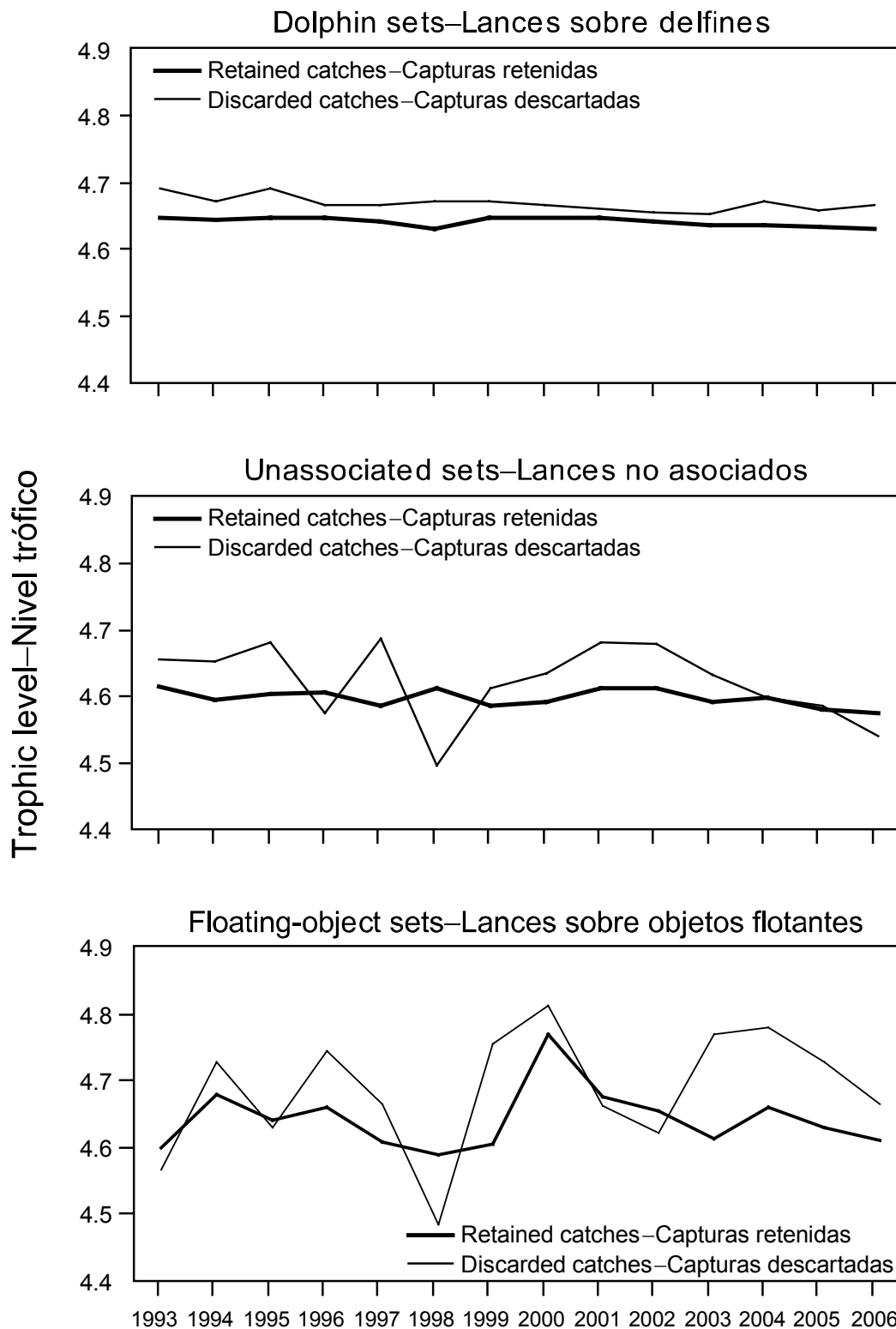
FIGURE J-4. Trophic level estimates of the retained catches and discarded catches by purse-seine fishing modes in the tropical eastern Pacific Ocean, 1993-2006. ESTIMATES FOR 2007 FORTHCOMING
