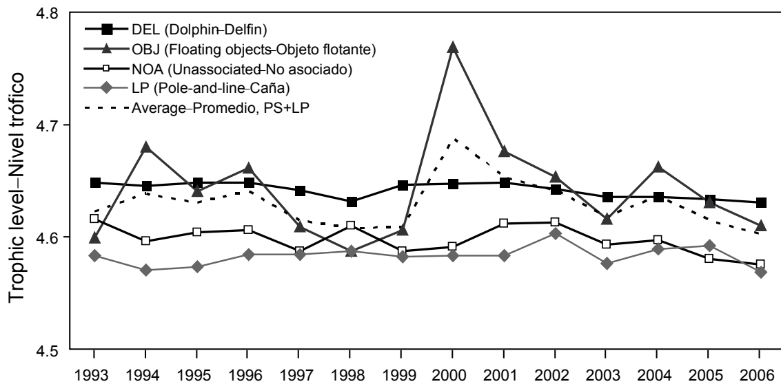
FIGURE J-2. Yearly trophic level estimates of the catches (retained and discarded) by the purse-seine and pole-and-line fisheries in the tropical eastern Pacific Ocean, 1993-2006. ESTIMATES FOR 2007 FORTHCOMING
