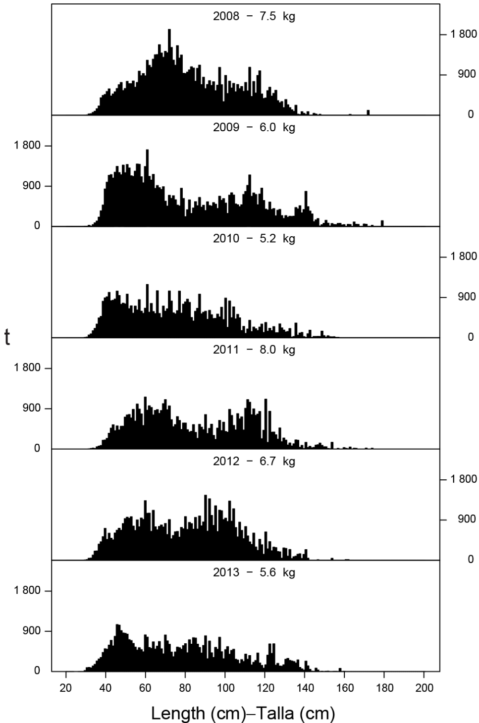
FIGURE A-8b. Estimated size compositions of the bigeye caught by purse-seine vessels in the EPO during 2008-2013. The average weights of the fish in the samples are given at the tops of the panels.
