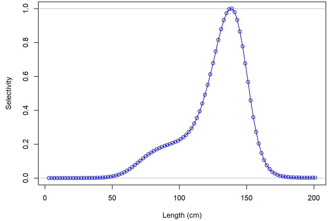
Female ending year selectivity for S1-PS_DEL_VAST
