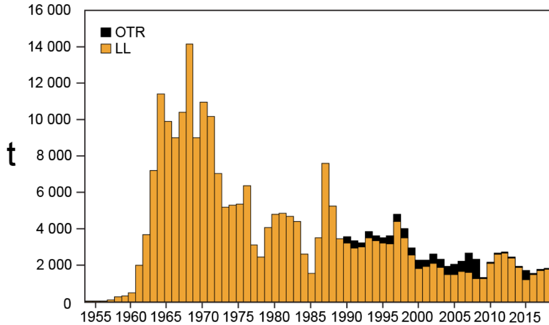
FIGURE I-1. Total reported catches of striped marlin in the North EPO by longline (LL) and other (OTR) fisheries (primarily recreational, 1954–2018). Due to unreported catches by recreational fisheries, estimates for 2009–2018 are minimums.
