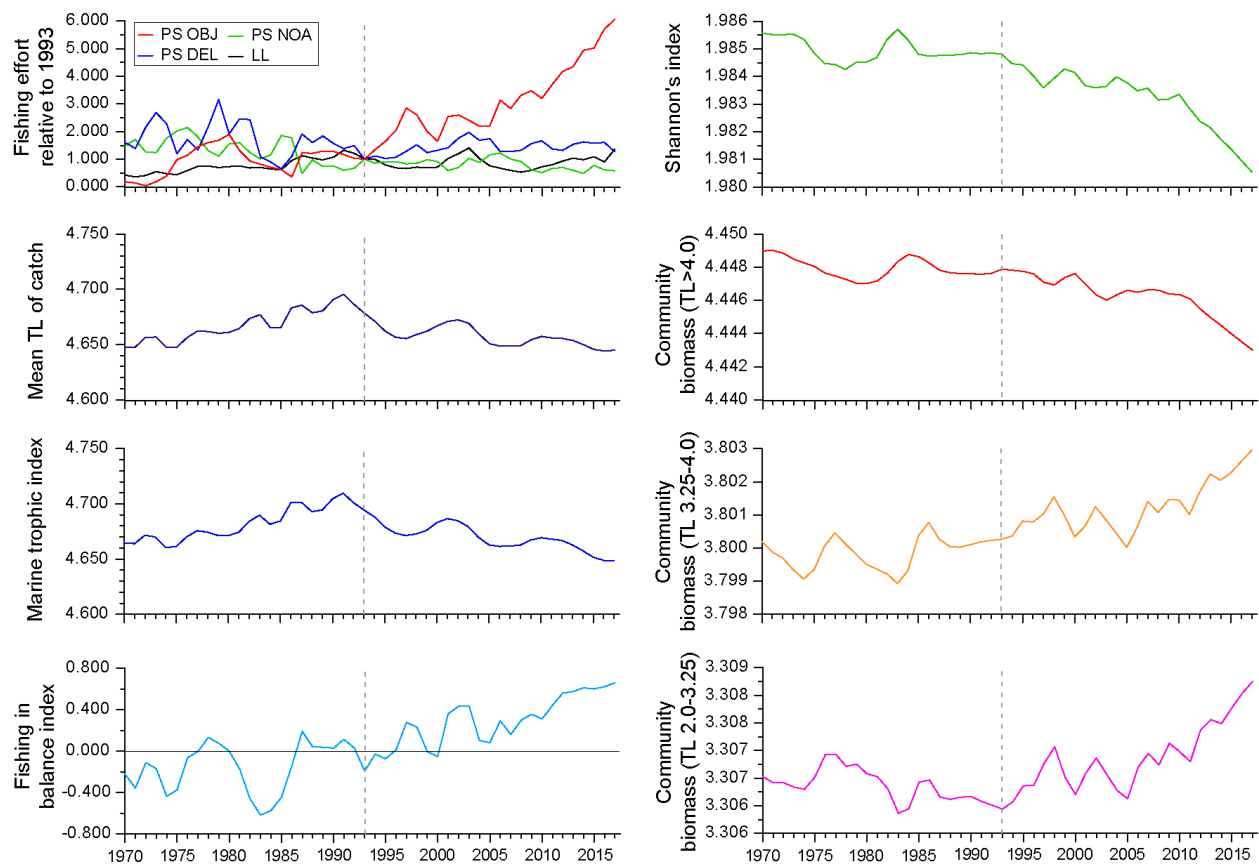
FIGURE L-13. Annual values for seven ecological indicators of changes in different components of the tropical EPO ecosystem, 1970–2017 (see Section 6 of text for details), and an index of longline (LL) and purse-seine (PS) fishing effort, by set type (dolphin (DEL), unassociated (NOA), floating object (OBJ)), relative to the model start year of 1993 (vertical dashed line), when the expansion of the purse-seine fishery on FADs began.
