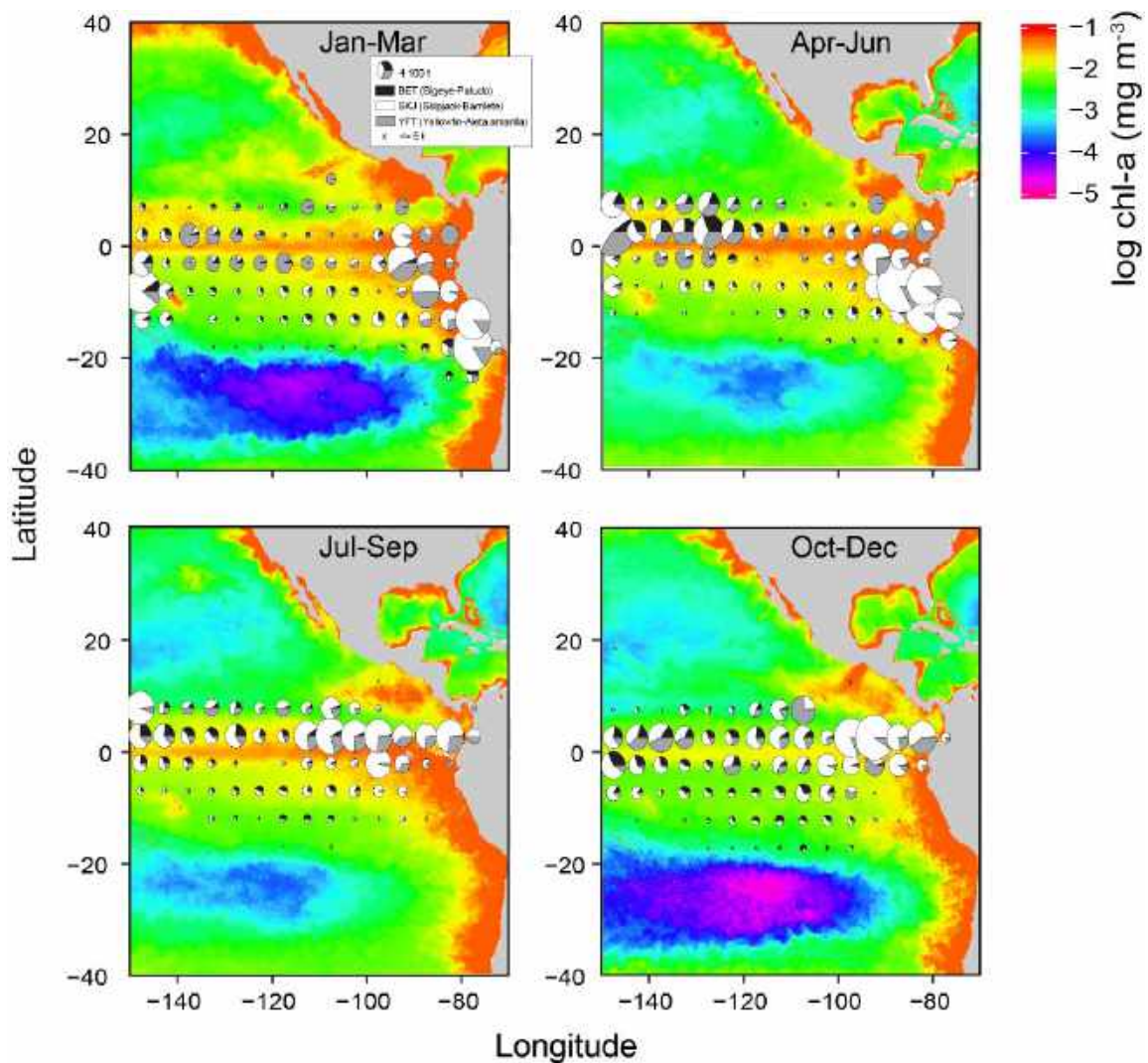
FIGURE L-11. Mean log chlorophyll-a concentration (in \text{mg m}^3 ) for each quarter during 2019 with catches of tropical tunas overlaid. Chlorophyll data obtained from NOAA CoastWatch on February 19, 2020, “Chlorophyll, NOAA, VIIRS, Science Quality, Global, Level 3, 2012-present, Monthly”, NOAA NMFS SWFSC ERD, https://coastwatch.pfeg.noaa.gov/erddap/info/nedisVHNSQchlaMonthly/index.html .
