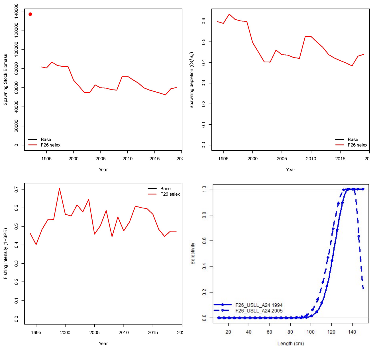
Figure 5.24. Estimated female spawning biomass (upper left), spawning depletion (upper right), fishing intensity (1-SPR) (lower left) for the 2020 base case model (black), where the size selectivity of the F26 US longline fishery was allowed to be dome-shaped (see Fig. 5.9), and a sensitivity run where the F26 fishery was forced to have an asymptotic selectivity (lower right). See Table 4.6 and Section 5.6.9 for details on sensitivity runs.
