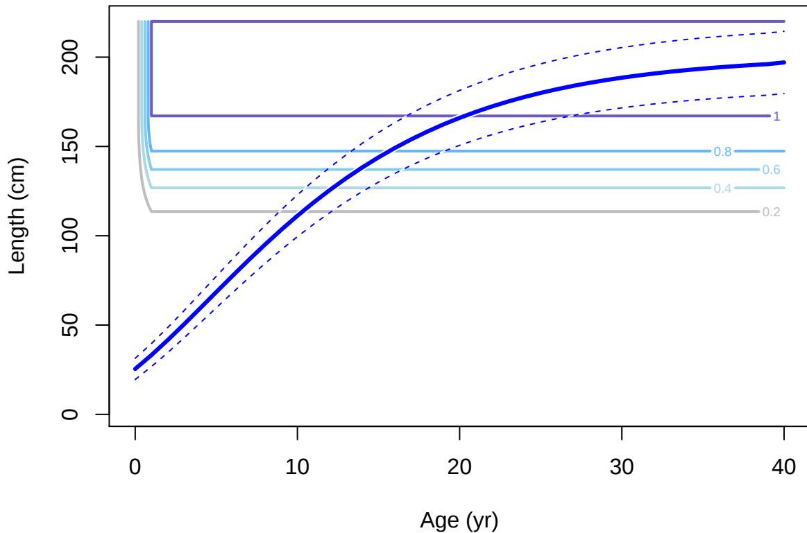
Male ending year selectivity and growth for A2-LL-w
