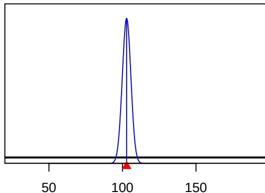
ze_DbIN_top_logit_F19-DEL_P(19)_BLK2repl_37
