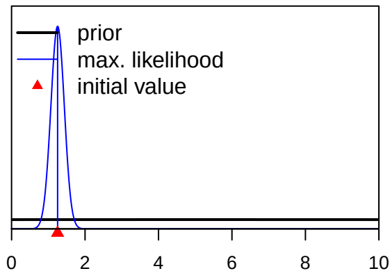
SizeSpline_GradHi_F12-NOA_C(12)
