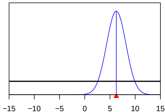
Size_DblN_descend_se_F19-DEL_P(19)
