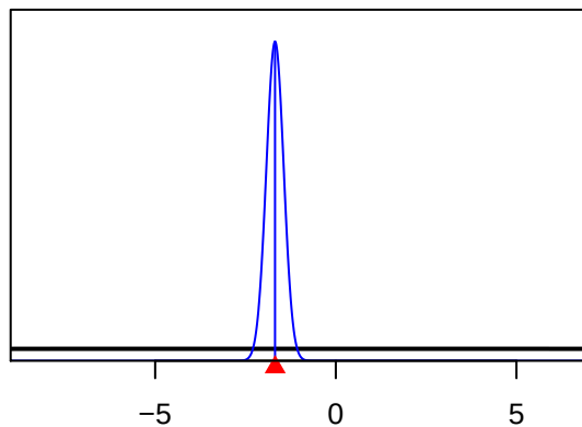
SizeSpline_Val_7_F11-NOA_N(11)
