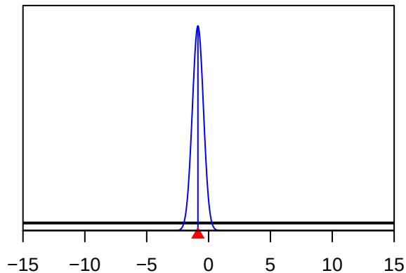
ze_DbIN_top_logit_F19-DEL_P(19)_BLK2repl_37
