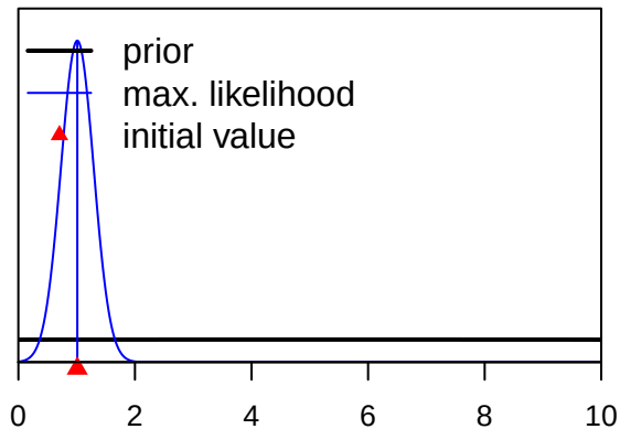
SizeSpline_GradHi_F13-NOA_I(13)
