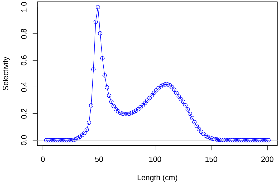
Female ending year selectivity for F4-OBJ_Cc_Q14
