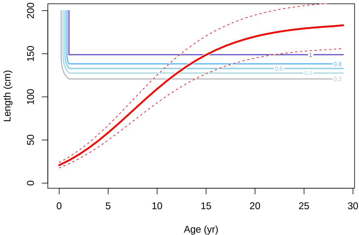
Female ending year selectivity and growth for F30-LL_C_Q14n
