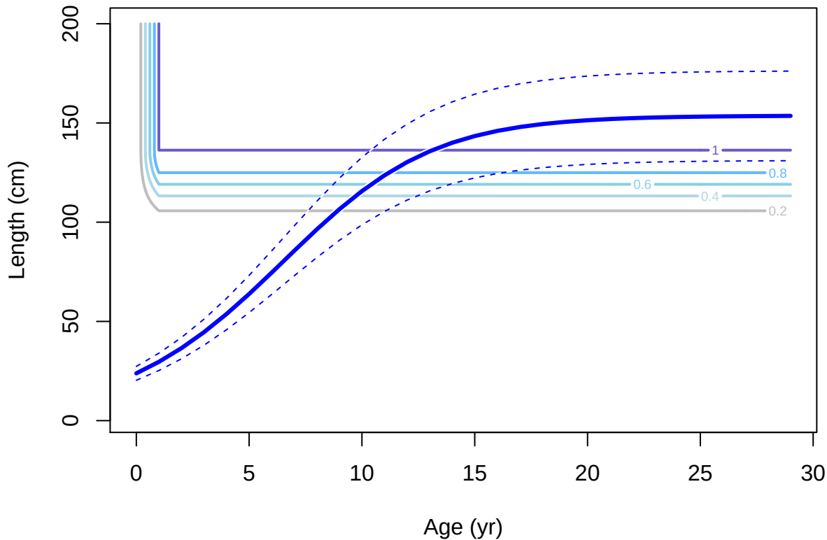
Male ending year selectivity and growth for F40-LL_E_Q23w
