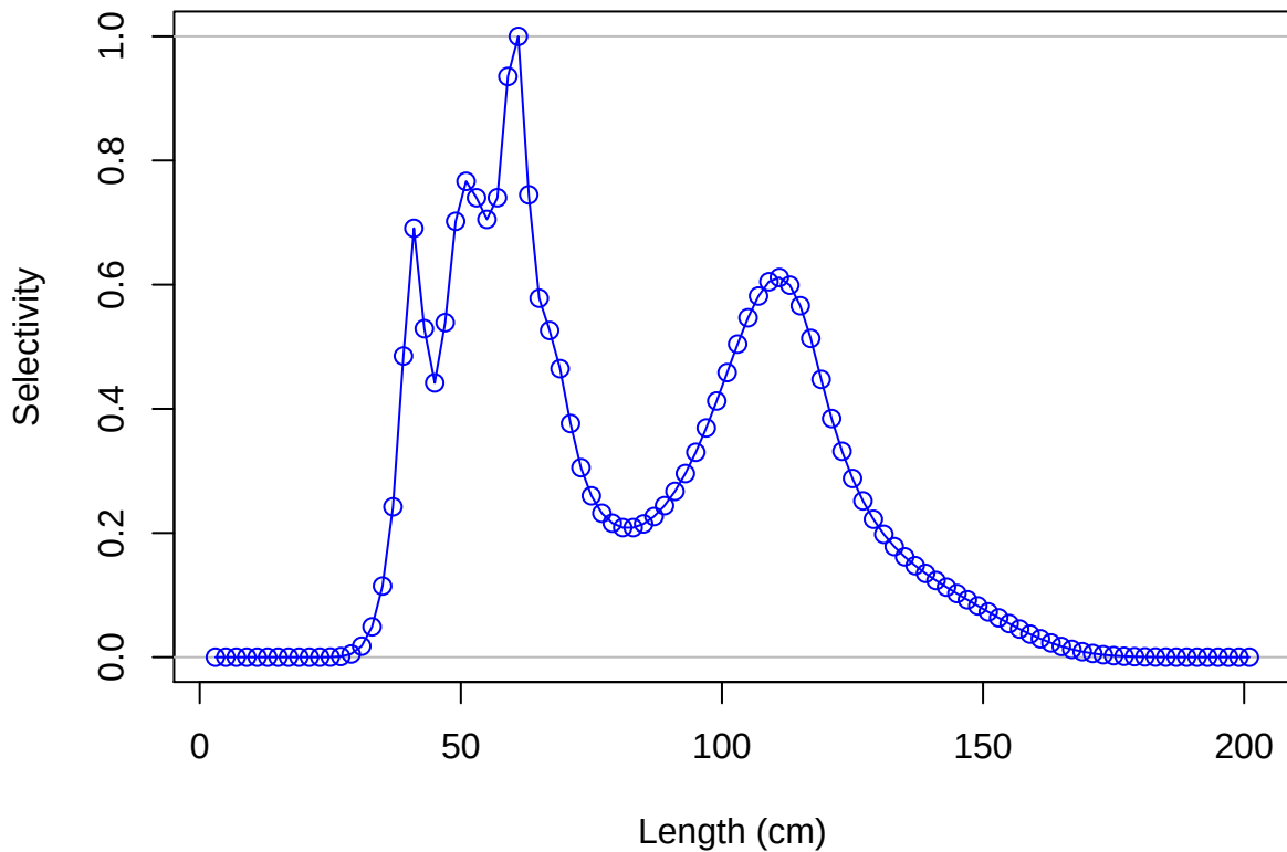
Female ending year selectivity for F8-OBJ_C_Q23
