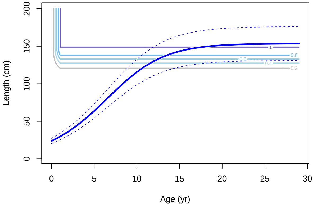
Male ending year selectivity and growth for F30-LL_C_Q14n
