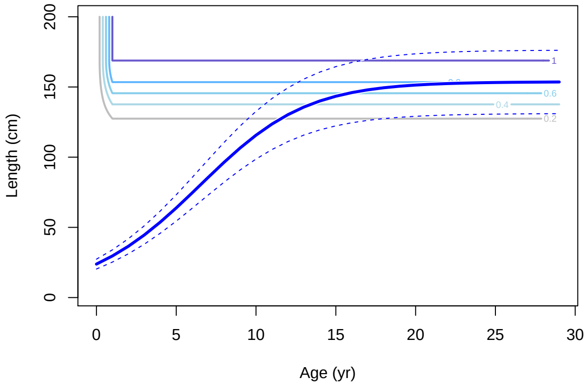
Male ending year selectivity and growth for F39-LL_C_Q23w
