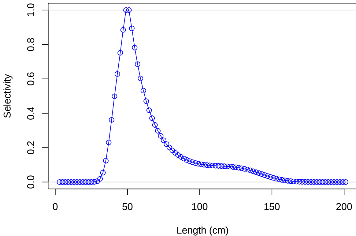
Female ending year selectivity for F6-OBJ_N_Q23
