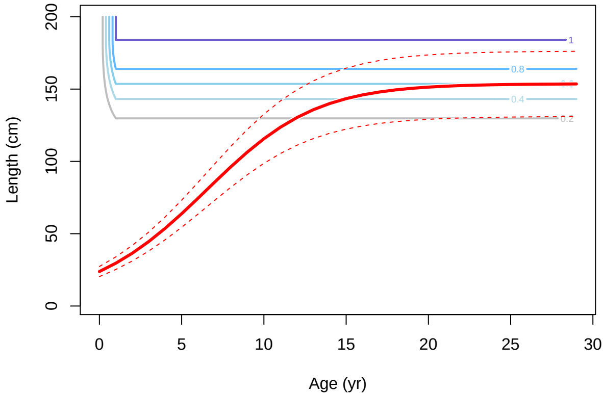
Female ending year selectivity and growth for F20-DEL_S
